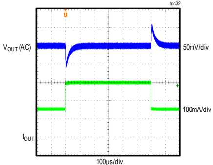
MAXM17901 LOAD TRANSIENT RESPONSE V_{IN} = 12V , FIXED V_{OUT} = 3.3V , PWM MODE (LOAD CURRENT STEPPED FROM 150mA TO 300mA)
