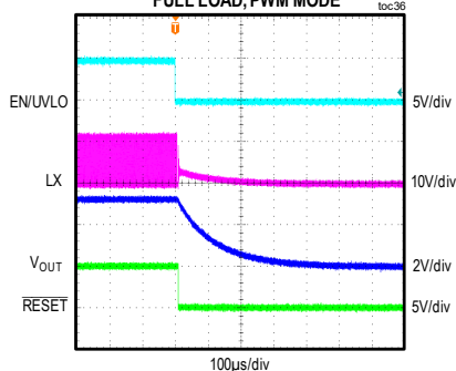
MAXM17903 SHUTDOWN THROUGH ENABLE V_{IN} = 12V , ADJUSTABLE V_{OUT} = 3.3V , FULL LOAD, PWM MODE
