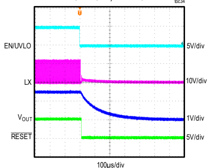
MAXM17903 SHUTDOWN THROUGH ENABLE V_{IN} = 12V , ADJUSTABLE V_{OUT} = 1.5V , FULL LOAD, PWM MODE
