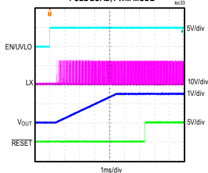
MAXM17903 STARTUP THROUGH ENABLE V_{IN} = 12V , ADJUSTABLE V_{OUT} = 1.5V , FULL LOAD, PWM MODE
