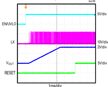
MAXM17903 STARTUP THROUGH ENABLE V_{IN} = 12V , ADJUSTABLE V_{OUT} = 3.3V , FULL LOAD, PWM MODE
