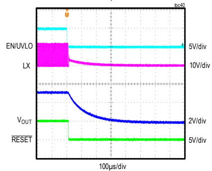
MAXM17901 SHUTDOWN THROUGH ENABLE V_{IN} = 12V , FIXED V_{OUT} = 3.3V , FULL LOAD, PWM MODE
