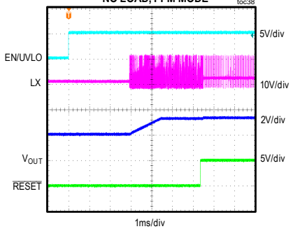
MAXM17903 STARTUP THROUGH ENABLE (2V PREBIAS) V_{IN} = 12V , ADJUSTABLE V_{OUT} = 3.3V , NO LOAD, PFM MODE
