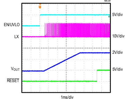
MAXM17901 STARTUP THROUGH ENABLE V_{IN} = 12V , FIXED V_{OUT} = 3.3V , FULL LOAD, PWM MODE
