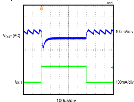
MAXM17903 LOAD TRANSIENT RESPONSE V_{IN} = 12V , ADJUSTABLE V_{OUT} = 3.3V , PFM MODE (LOAD CURRENT STEPPED FROM 5mA TO 150mA)
