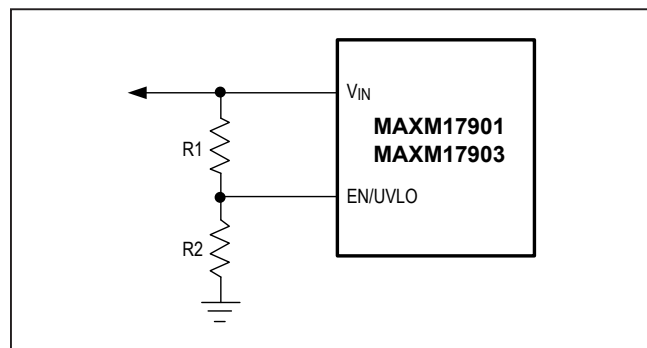
Figure 1. Adjustable EN/UVLO Network
