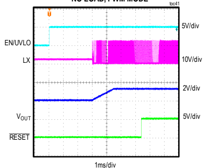
MAXM17901 STARTUP THROUGH ENABLE (2V PREBIAS) V_{IN} = 12V , FIXED V_{OUT} = 3.3V , NO LOAD, PWM MODE
