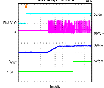
MAXM17901 STARTUP THROUGH ENABLE (2V PREBIAS) V_{IN} = 12V , FIXED V_{OUT} = 3.3V , NO LOAD, PFM MODE
