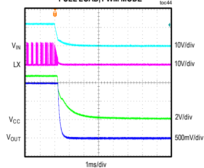
MAXM17903 SHUTDOWN THROUGH V_{IN} V_{IN} = 12V , ADJUSTABLE V_{OUT} = 1.5V , FULL LOAD, PWM MODE
