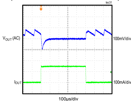
MAXM17901 LOAD TRANSIENT RESPONSE V_{IN} = 12V , FIXED V_{OUT} = 3.3V , PWM MODE (LOAD CURRENT STEPPED FROM 5mA TO 150mA)
