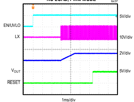
MAXM17903 STARTUP THROUGH ENABLE (2V PREBIAS) V_{IN} = 12V , ADJUSTABLE V_{OUT} = 3.3V , NO LOAD, PWM MODE
