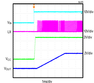
MAXM17903 STARTUP THROUGH V_{IN} V_{IN} = 12V , ADJUSTABLE V_{OUT} = 3.3V , FULL LOAD, PWM MODE
