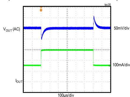
MAXM17903 LOAD TRANSIENT RESPONSE V_{IN} = 12V , ADJUSTABLE V_{OUT} = 3.3V , PWM MODE (LOAD CURRENT STEPPED FROM 150mA TO 300mA)
