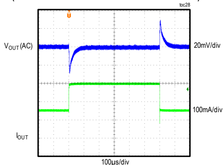
MAXM17903 LOAD TRANSIENT RESPONSE V_{IN} = 12V , ADJUSTABLE V_{OUT} = 1.5V , PWM MODE (LOAD CURRENT STEPPED FROM 150mA TO 300mA)
