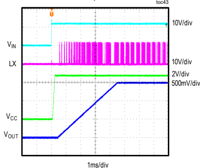
MAXM17903 STARTUP THROUGH V_{IN} V_{IN} = 12V , ADJUSTABLE V_{OUT} = 1.5V , FULL LOAD, PWM MODE
